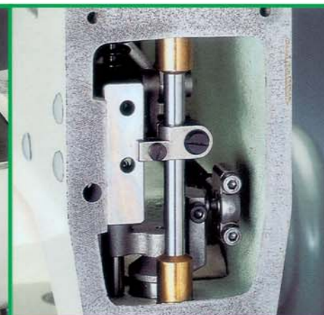
针柱固定滑板之设计，使针柱不易晃动，押脚心结构改良。 The needle fixator keeps the needle from vibration while the platen core comes with a modified mechanism.
